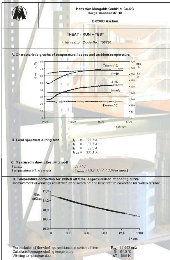
Fig. 6: Heat-run test report
