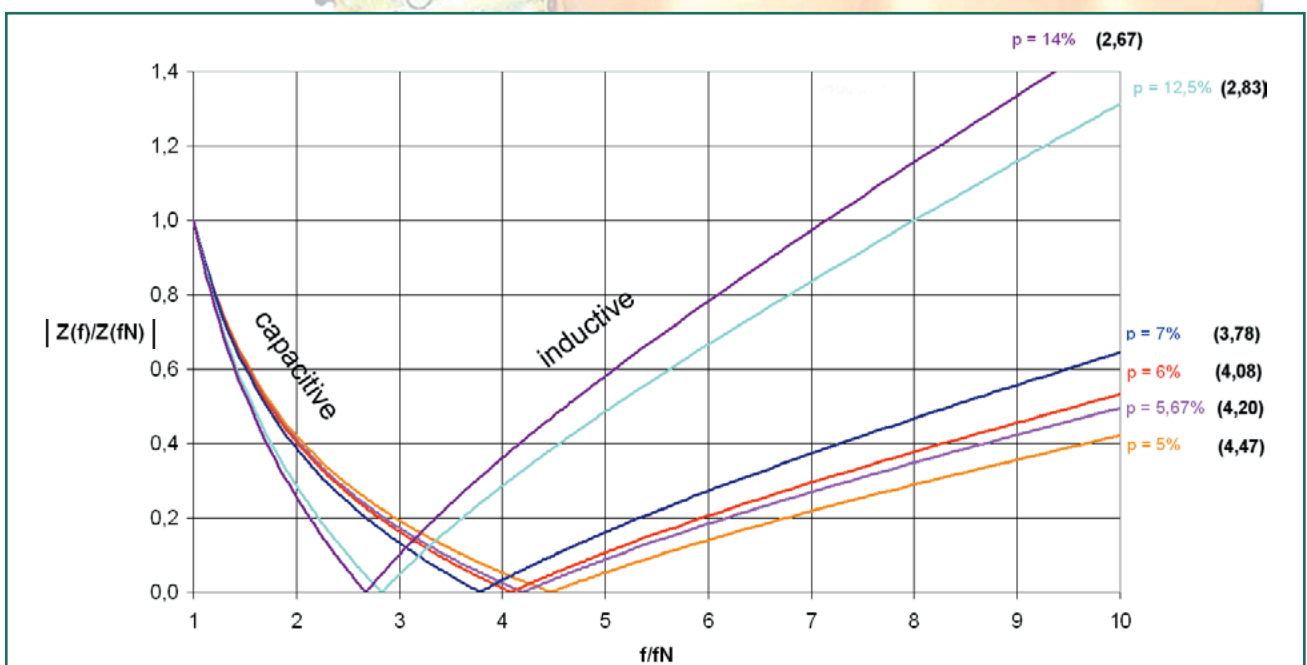
Fig. 1: Common detuning factors and ordinal of resonance
